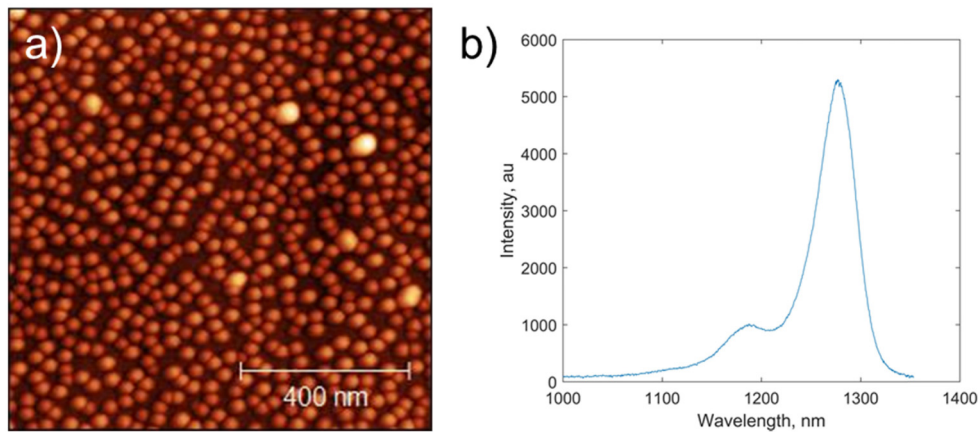
Fig. 4. (a) Atomic force microscope image of a 1 \times 1 \mu\text{m}^2 region of quantum dots showing a total dot density of 6 \times 10^{10} \text{ cm}^{-2} . (b) A photoluminescence spectrum for the quantum dots grown on a native GaAs substrate with conditions identical to those used for the laser showing a peak wavelength of 1277 nm and full-width at half-maximum of 36 meV.
